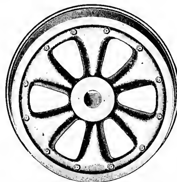
Figs. 5272-5273. Wheel with Cast-iron Spoke-center. Tire shrunk on Center.
